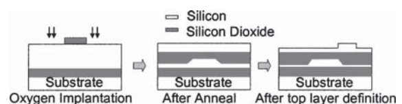
FIG. 1. Process flow for the SIMOX fabrication of 3-D structures (cross-sectional view).
